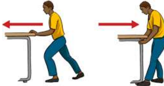
Gambar 15. Ilustrasi Gaya (Sumber: https://www.google.com/search )
