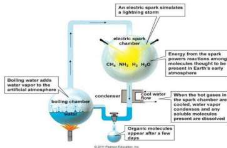
Gambar 75. Percobaan Miller – Urey
