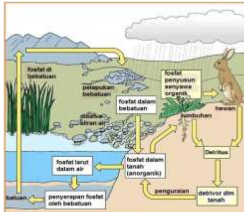
Gambar 151. Siklus Fosfor (Campbell, Reece & Mitchell, 2004)
