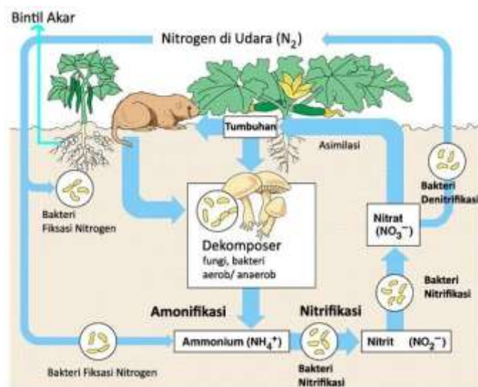
Gambar 150. Siklus nitrogen (Campbell, Reece & Mitchell, 2004)
